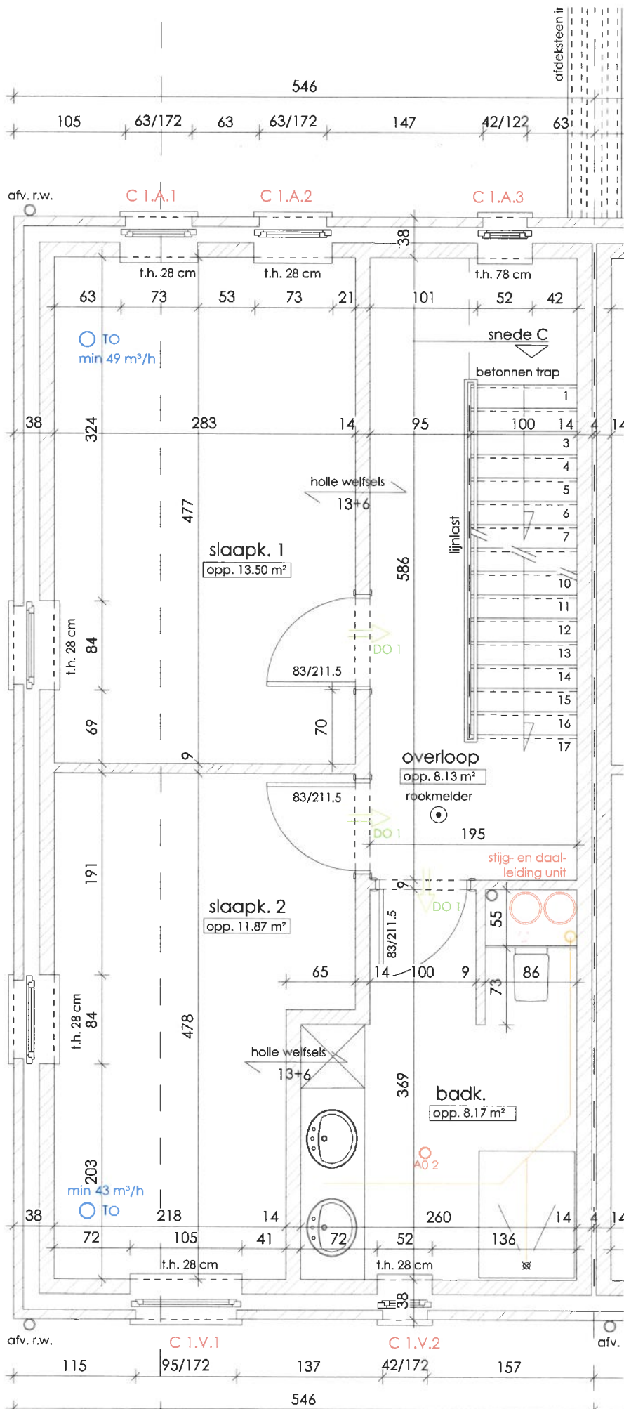
plan verdieping
