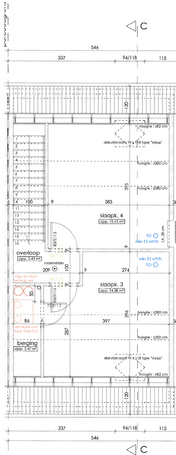
plan zolder woning B6 opp. zolder : 47.42 m 2
