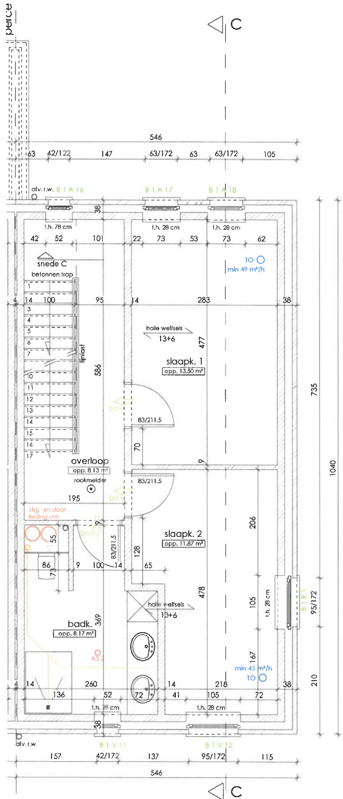
plan verdieping woning B6 opp. verdieping : 56.78 m²
