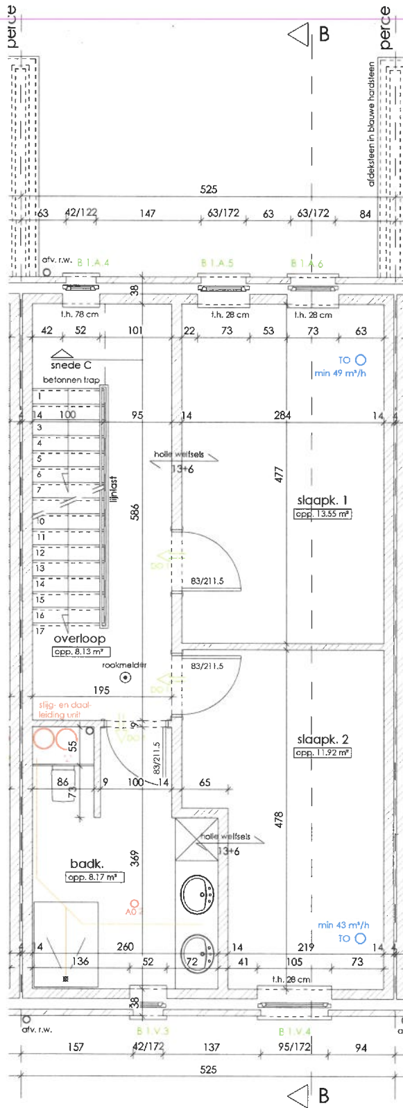
plan verdieping woning B2 opp. verdieping : 54.60 m²
