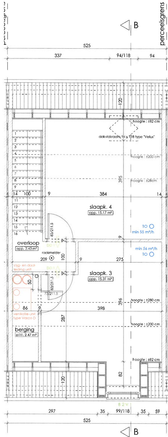
plan zolder woning B2 opp. zolder : 47.05 m 2
