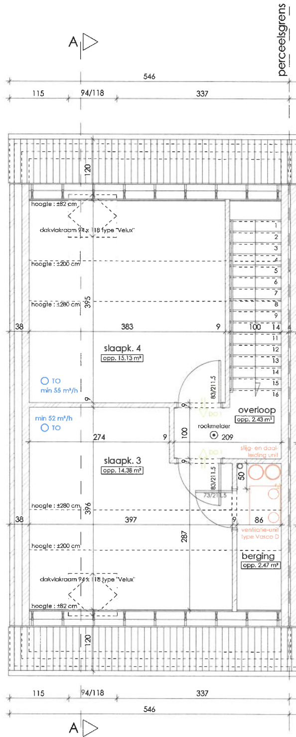
plan zolder woning B1 opp. zolder : 47.42 m²
